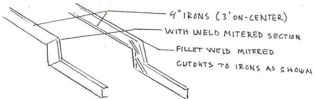
WELDING DETAIL
